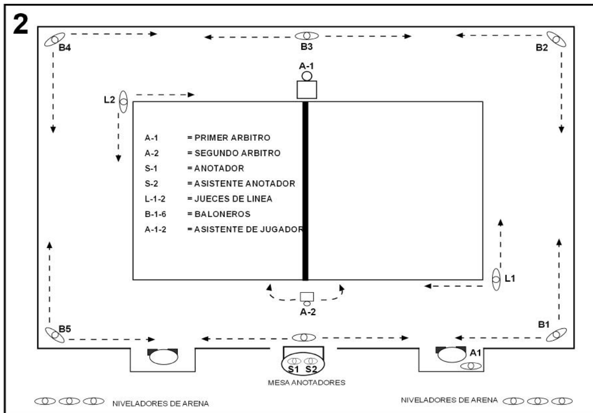
SUPPORT PERSONAL POSITION / LOCALIZACION DEL PERSONAL. FIG.2
